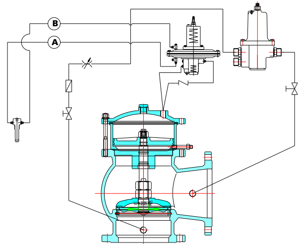
Angle Pattern DN 40-300
