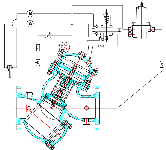
Filter Version DN 40-300
